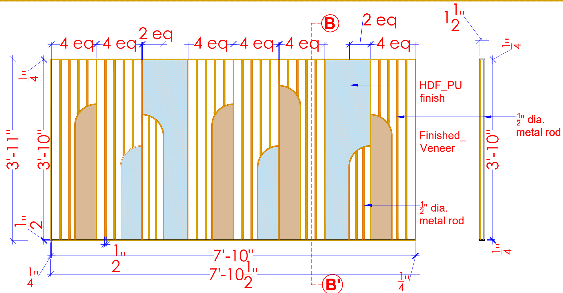
SECTION BB'
